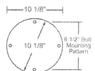
Bolt Circle Pattern For 4" Posts Anchor Bolt 3/4" x 18"
